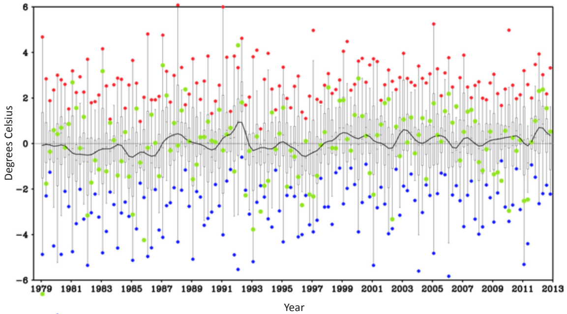
Figure A3. Same as Figure A2, except for surface air temperature anomalies ( ^{\circ}\text{C} ).
