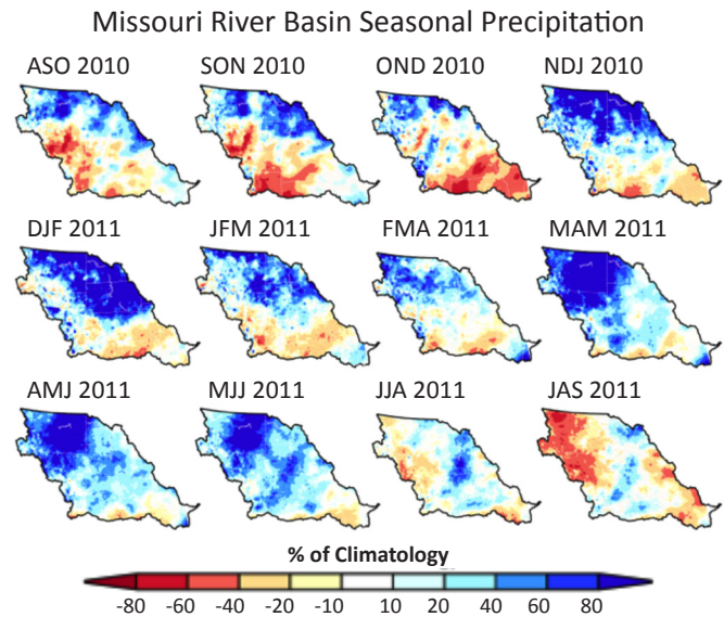
Figure 12. Observed Missouri Basin seasonal precipitation departures (% above or below climatology) from August-October 2010 (top left) thru July-September 2011 (lower right). Anomalously wet (dry) areas denoted in blue (red) shades. Climatological reference is period of record 1895-2012. Precipitation data source is PRISM.
