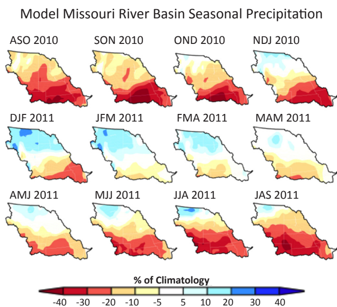
Figure 16. Model simulated Missouri Basin seasonal precipitation departures (% above or below climatology) from August-October 2010 (top left) thru July-September 2011 (lower right). Anomalously wet (dry) areas denoted in blue (red) shades. Climatological reference is based on the ECHAM5 model simulation period of record 1979-2012. Precipitation data is based on the 40-member ensemble averaged of the ECHAM5 simulations.
