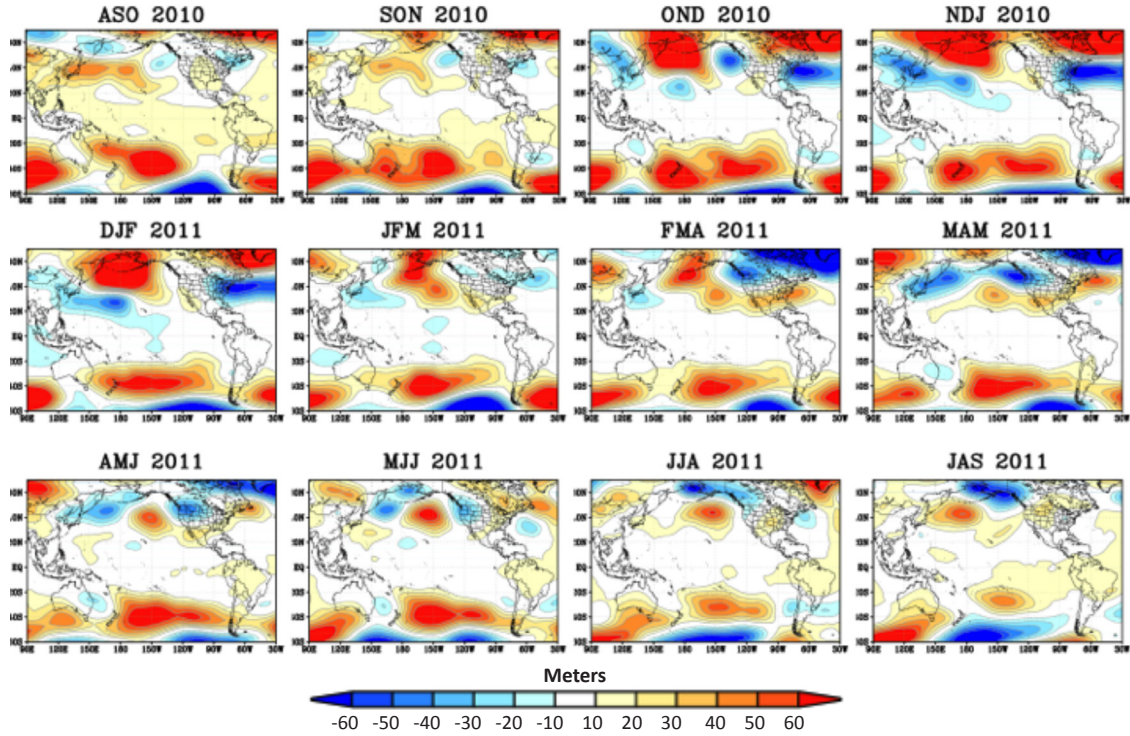
Figure 14. Observed seasonal 500 mb height anomalies (m) for August-October 2010 (top left) thru July-September 2011 (lower right). Anomalously low (high) pressure areas denoted in blue (red) shades. Departures are relative to period of record 1948-2012. The 500 mb height data is based on NCEP/NCAR reanalysis.
