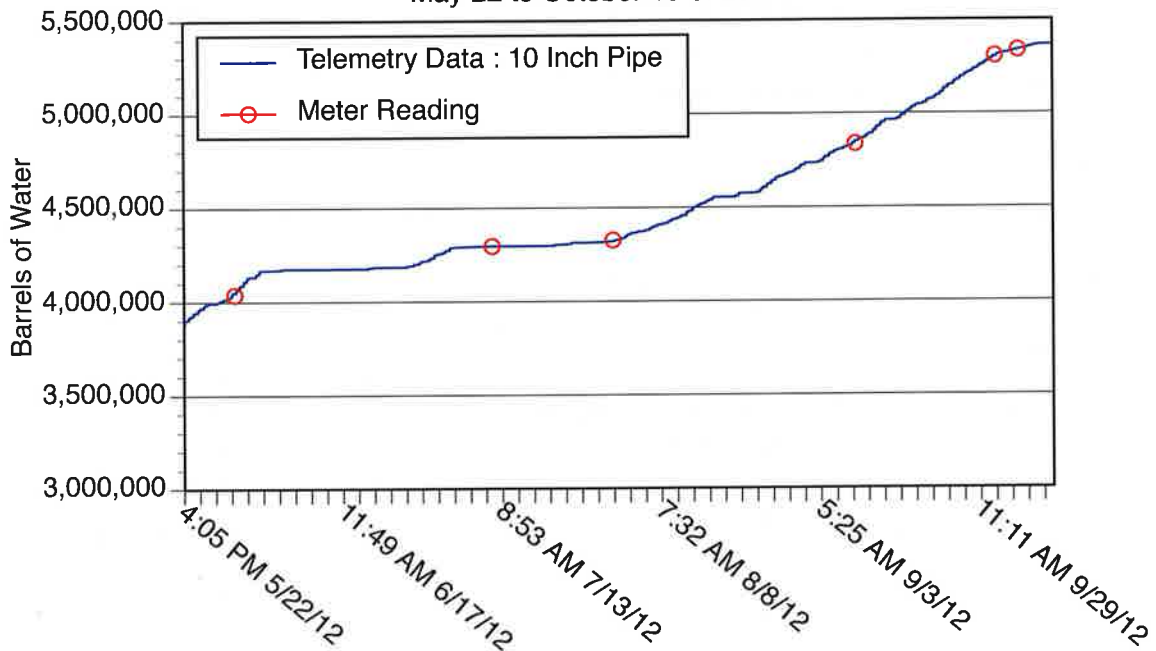
Steve Mortenson : Trenton Water Depot : 10 Inch Pipe Telemetry Data (every 6 hours) & Meter Readings (single observations) May 22 to October 10 of 2012
