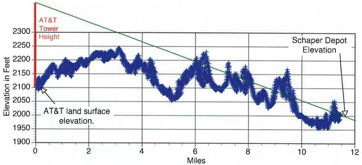
Line-of-Sight plot, from AT&T tower to Schaper Depot, using DEM data (~400 feet wide).
