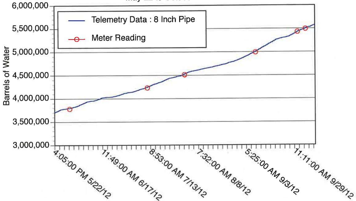
Steve Mortenson : Trenton Water Depot : 8 Inch Pipe Telemetry Data (every 6 hours) & Meter Readings (single observations) May 22 to October 10 of 2012
