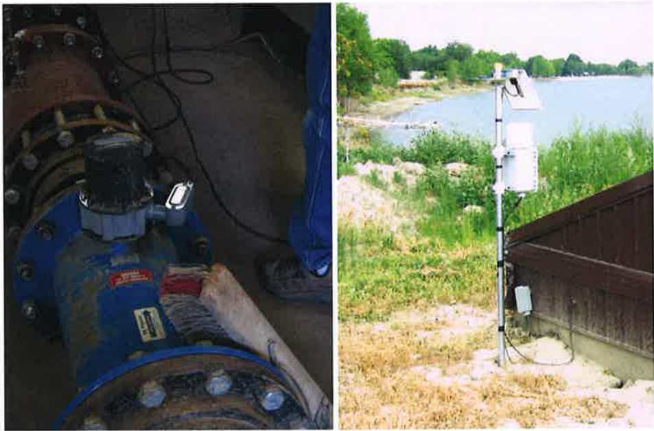
Figure 3. Installation of McCrometer Telemetry at the Trenton Water Depot owned by Steve Mortenson. (LEFT) Pulse counter installed on McCrometer Meter : (RIGHT) Exterior installation of telemetry system
