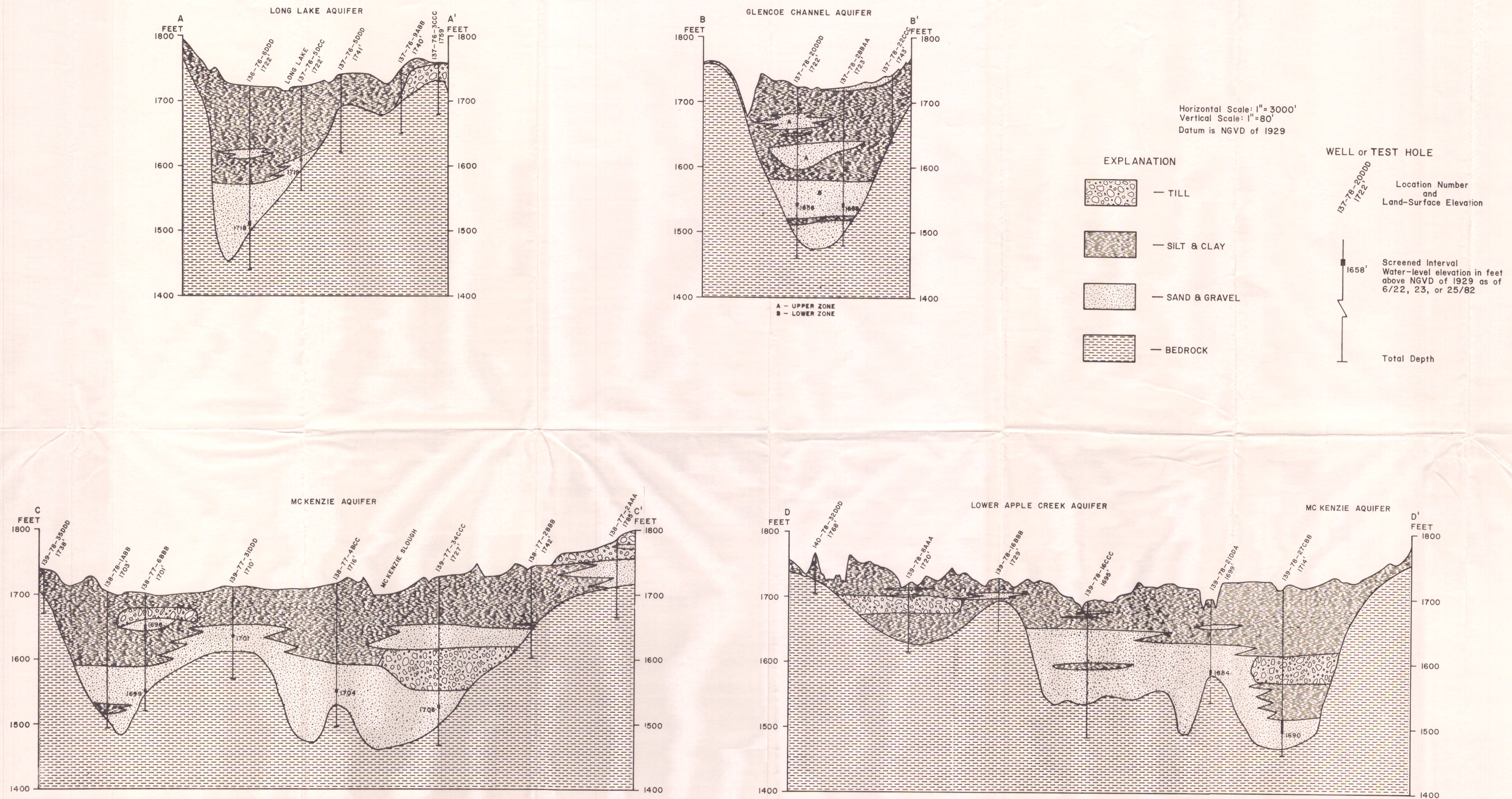
PLATE 9. HYDROGEOLOGIC CROSS-SECTIONS SHOWING GLACIAL-DRIFT AQUIFERS—BURLEIGH COUNTY Hydrogeology by D. R. Larson, 1985
