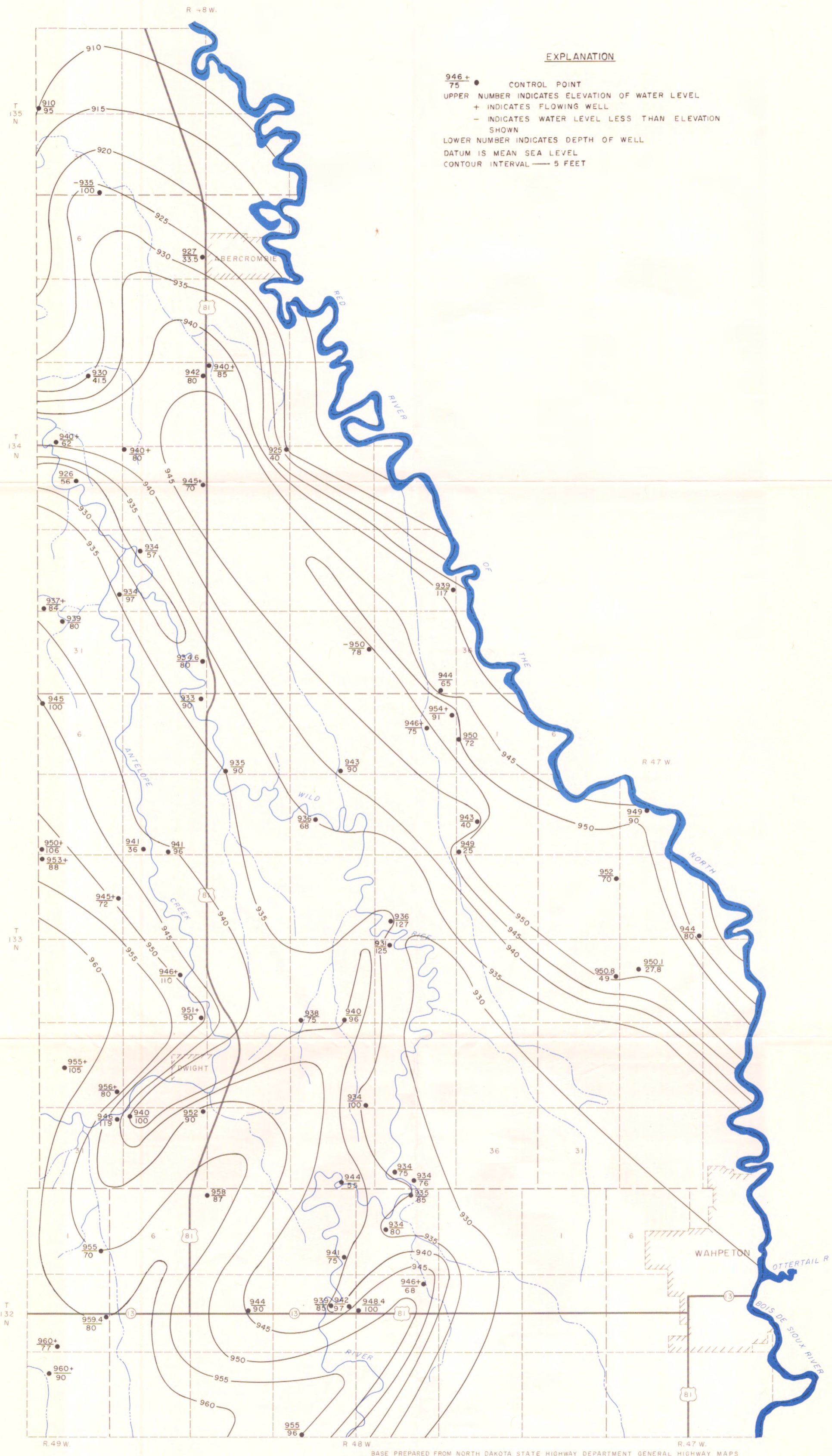
PLATE 6 -- MAP SHOWING CONFIGURATION OF THE POTENTIOMETRIC SURFACE OF THE WAHPETON SAND-PLAIN AQUIFER
