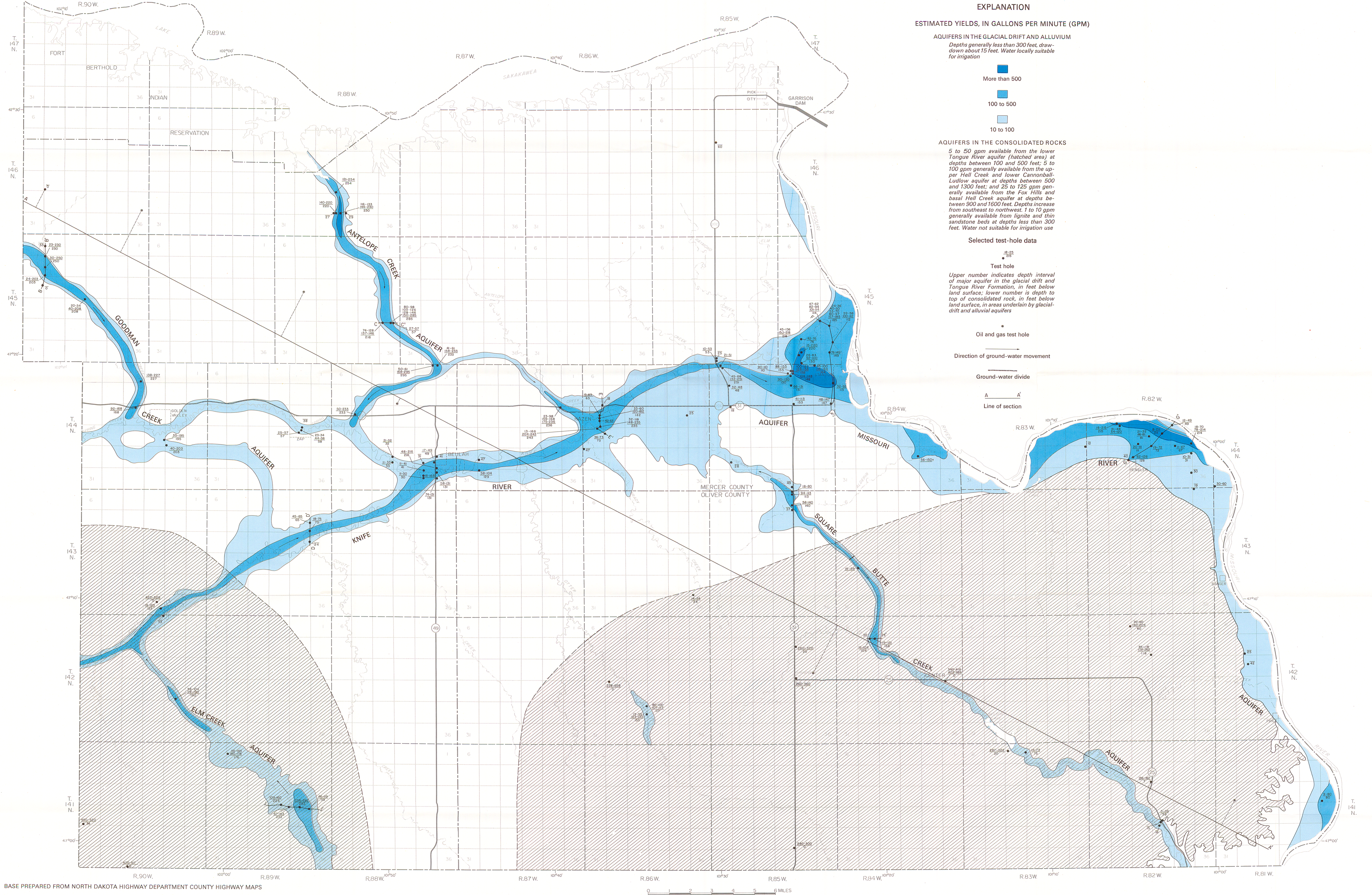
PLATE 1.—MAP SHOWING AVAILABILITY OF GROUND WATER IN MERCER AND OLIVER COUNTIES, NORTH DAKOTA
