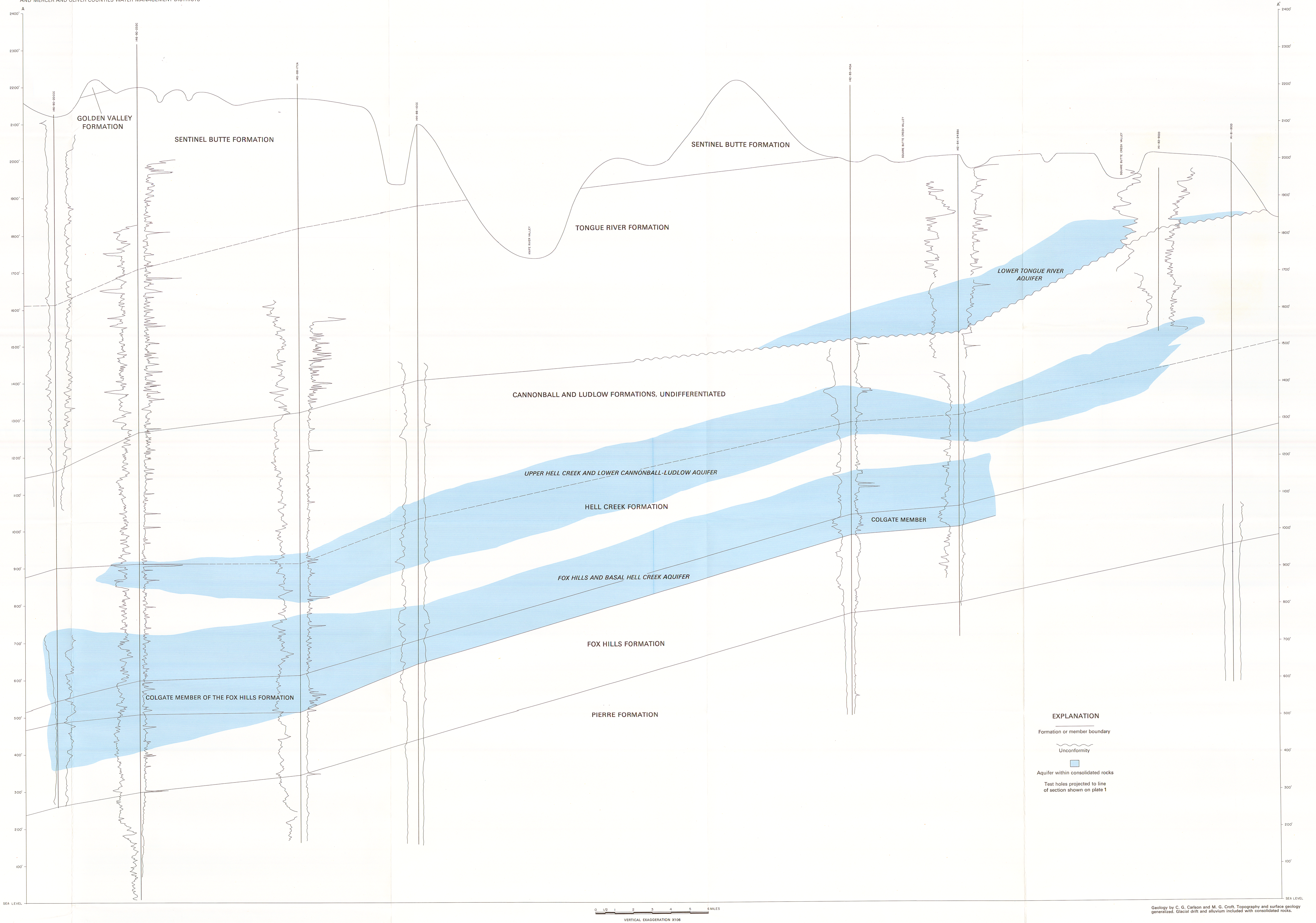
PLATE 2.—HYDROGEOLOGIC SECTION A-A', MERCER AND OLIVER COUNTIES, NORTH DAKOTA
