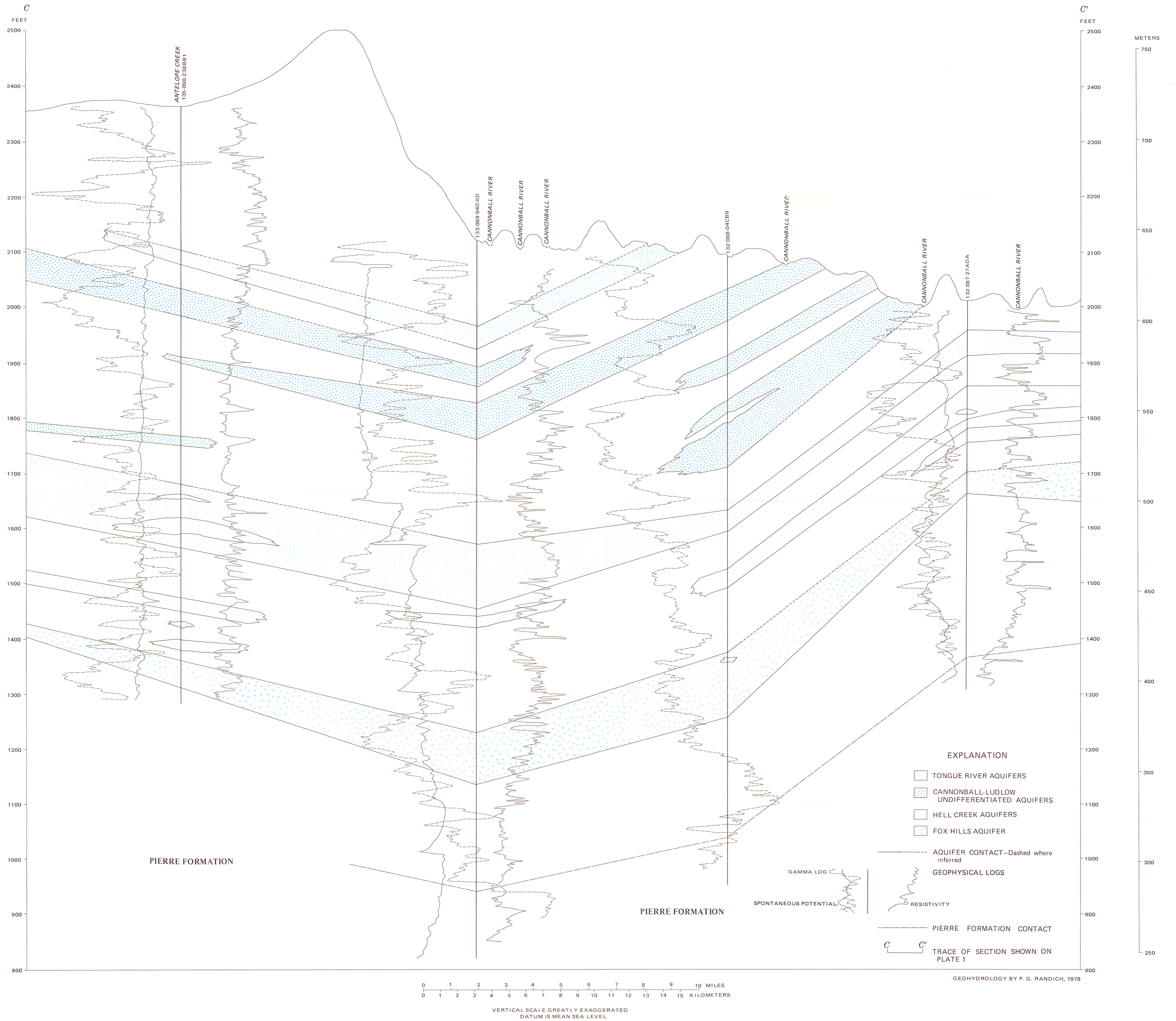
PLATE 4.—GEOHYDROLOGIC SECTION C-C' SHOWING SYNCLINAL STRUCTURE AND BEDROCK AQUIFERS, GRANT AND SIOUX COUNTIES, NORTH DAKOTA
