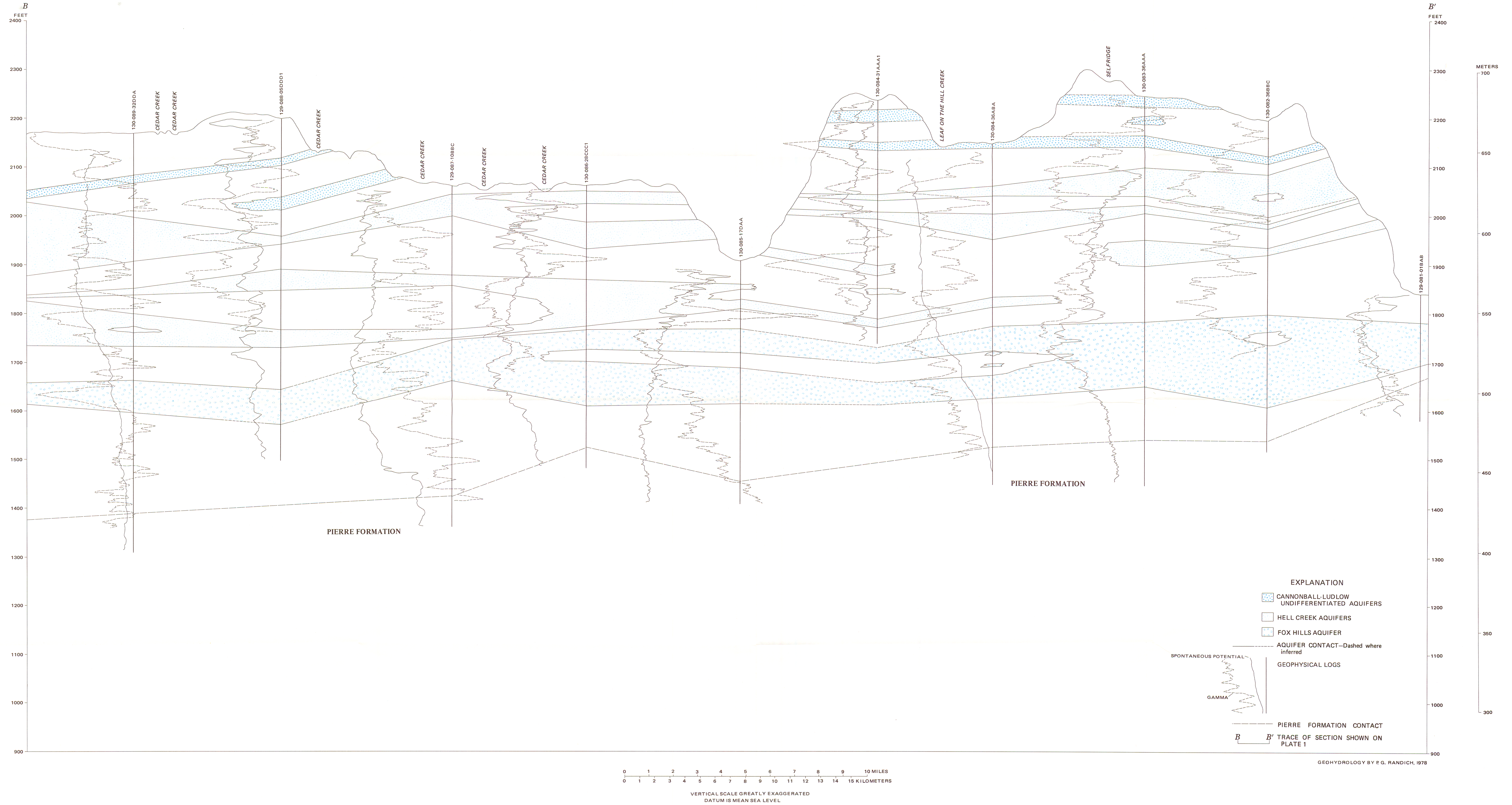
PLATE 3.—GEOHYDROLOGIC SECTION B-B' SHOWING BEDROCK AQUIFERS, GRANT AND SIOUX COUNTIES, NORTH DAKOTA
