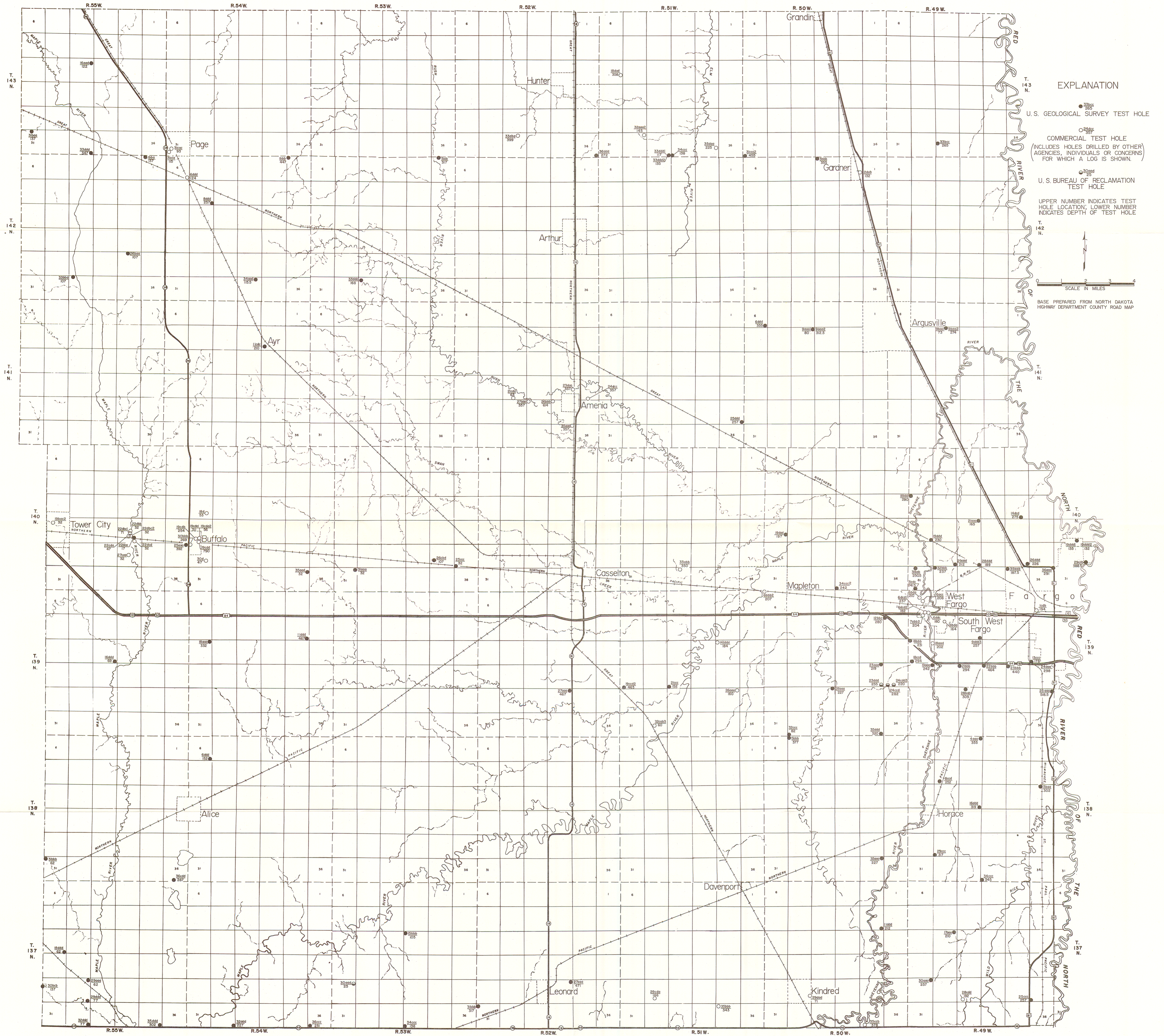
FIGURE 4. MAP SHOWING LOCATION OF TEST HOLES IN CASS COUNTY
